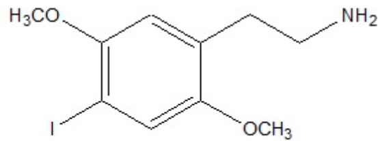
4-Iodo-2,5-dimethoxybenzeneethanamine
