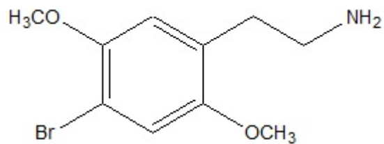
4-Bromo-2,5-dimethoxybenzeneethanamine
